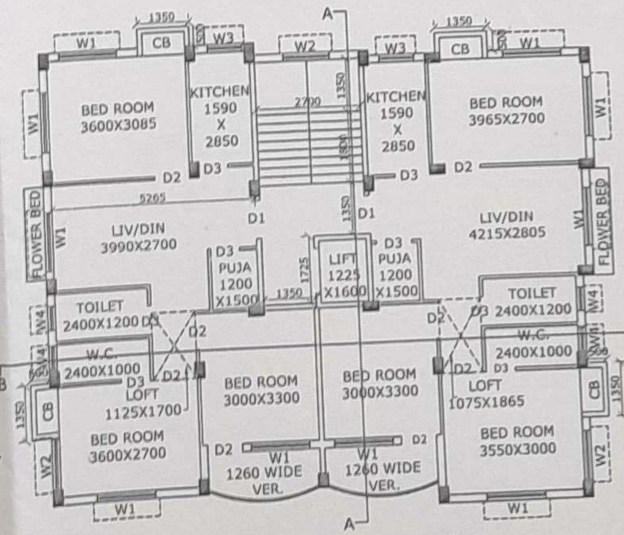
1ST, 2ND & 4TH FLOOR PLAN
