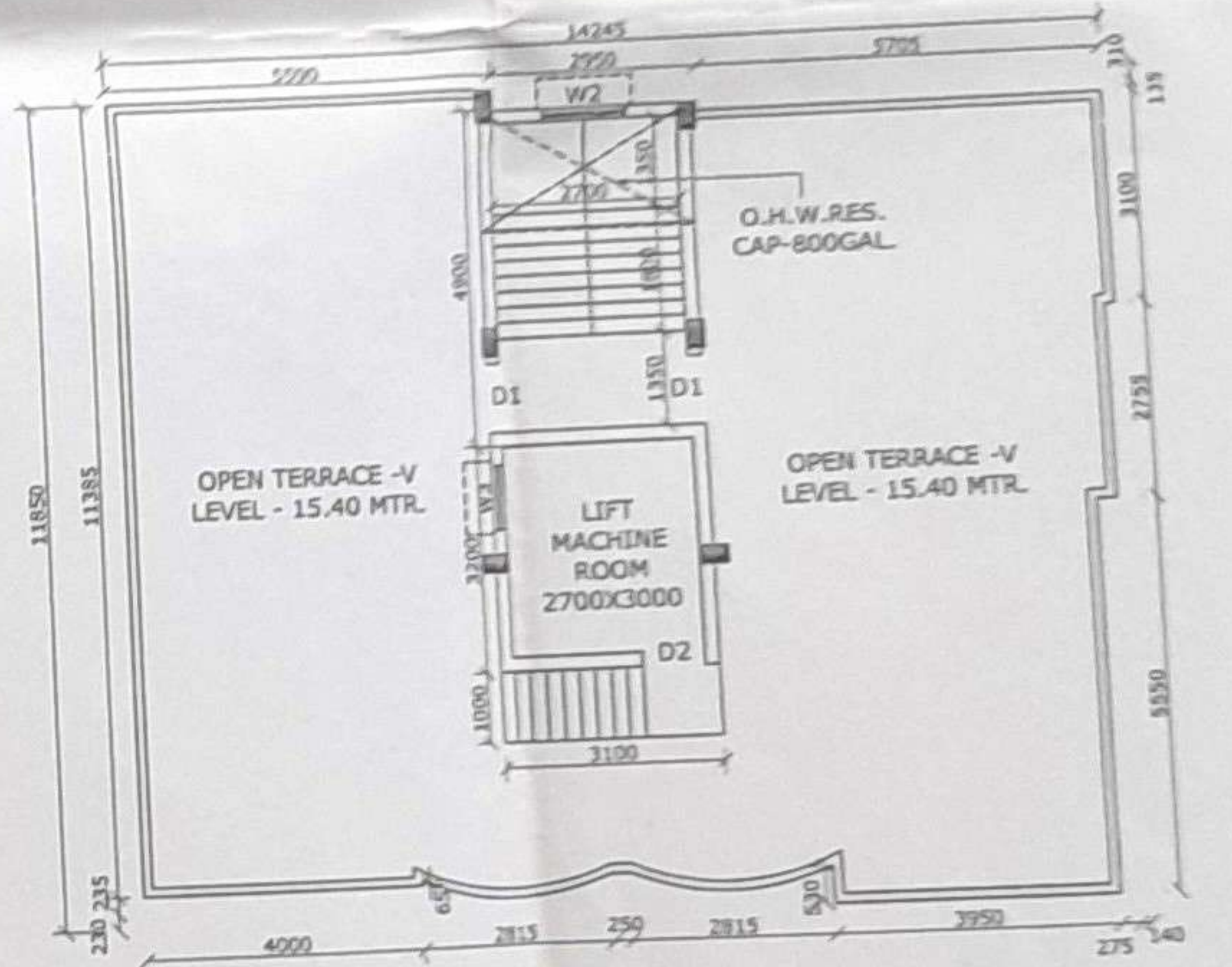
ROOF PLAN
